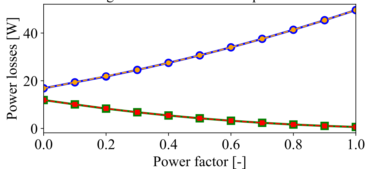
Average IGBT and diode total power losses
