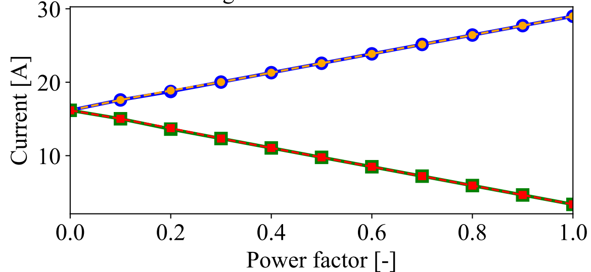
Average IGBT and diode current
