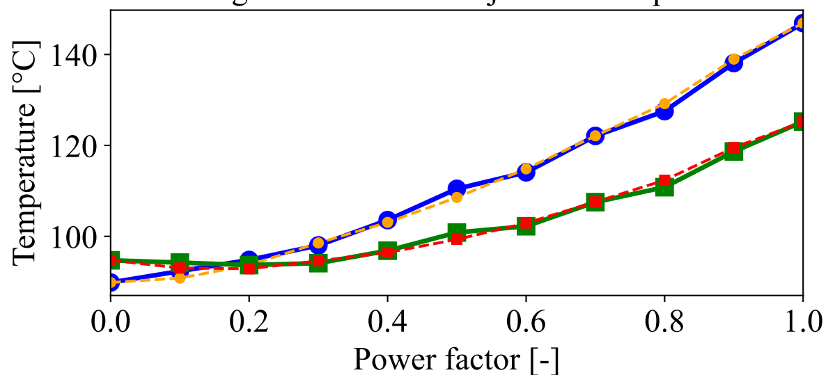
Average IGBT and diode junction temperature
