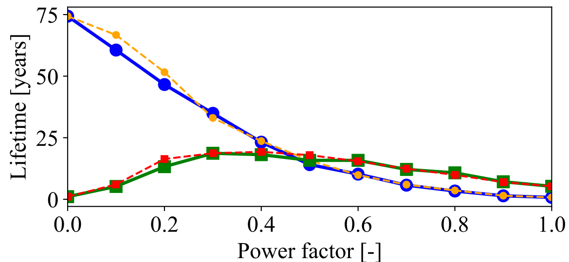
IGBT and diode estimated lifetime
